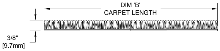
SECTION Y-Y
