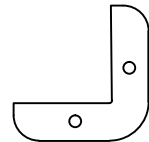
SMWS-10 END CAP STAINLESS STEEL (24S084000) WOOD (24W339xxx)
