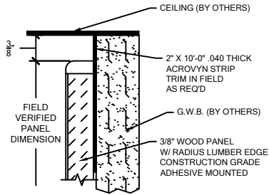
CEILING REVEAL
