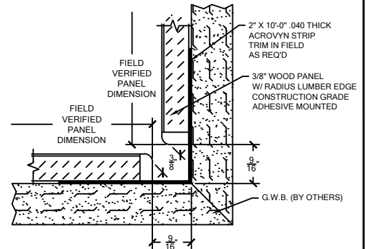
INSIDE CORNER CONDITION
