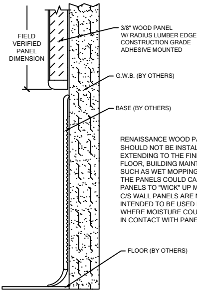
BASE CONDITION
