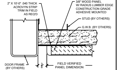
END REVEAL
