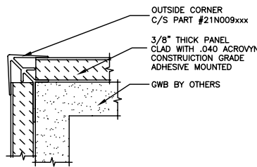
OUTSIDE CORNER QTY REQ'D. _____
