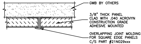
SQUARE EDGE JOINT MOLDING QTY REQ'D. _____
