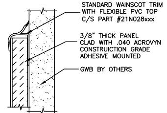
WAINSCOT TRIM QTY REQ'D. _____
