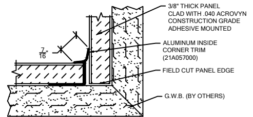
ALUMINUM INSIDE CORNER TRIM QTY.: _____
