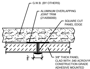
ALUMINUM OVERLAPPING JOINT TRIM QTY.: _____
