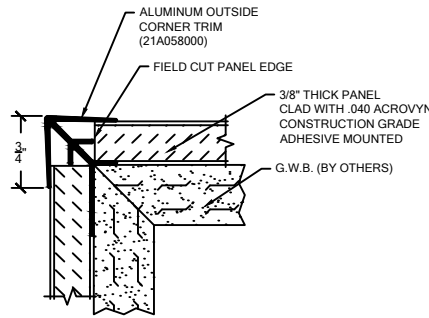
ALUMINUM OUTSIDE CORNER TRIM QTY.: _____
