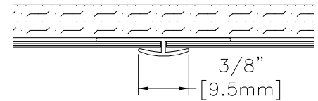
"H" JOINT MOLDING (25N033XXX)
