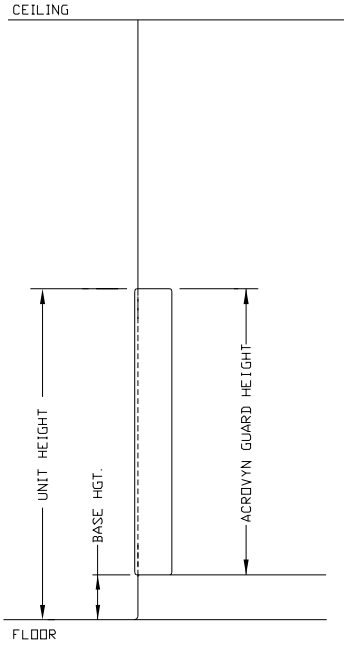
VA-250 GUARD AT PARTIAL HEIGHT ELEVATION
