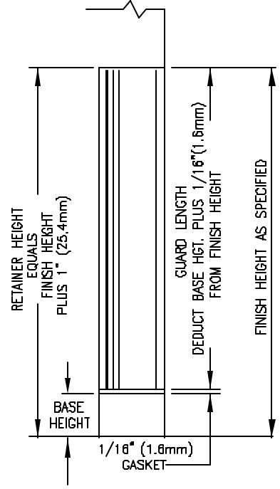
FLUSH MOUNTED GUARD AT PARTIAL HEIGHT ELEVATION
