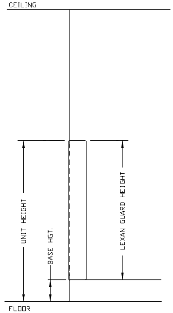
LG-150 GUARD AT PARTIAL HEIGHT ELEVATION
