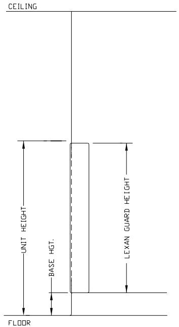
LG-118M GUARD AT PARTIAL HEIGHT ELEVATION
