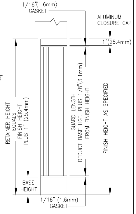
FLUSH MOUNTED GUARD AT PARTIAL HEIGHT ELEVATION
