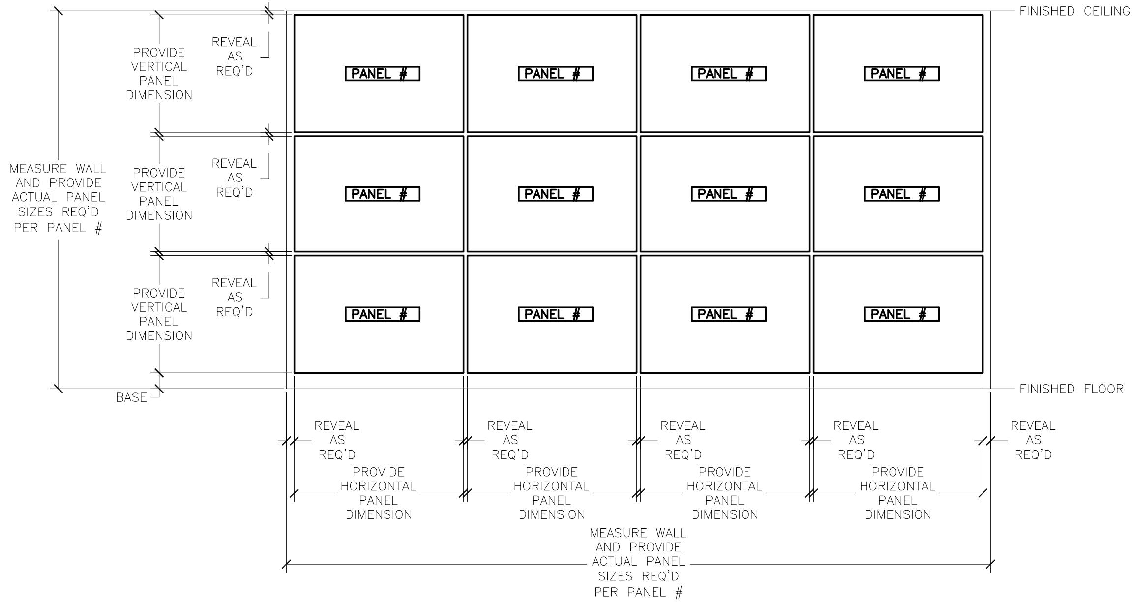
TYPICAL PANEL ELEVATION 1/2" = 1'-0"
